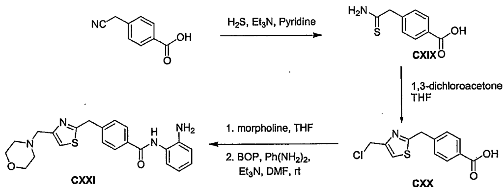
Scheme 42
